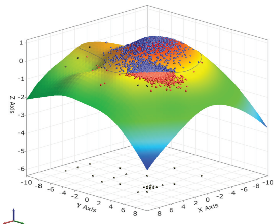
Adaptive response surface for estimating the probability of exceeding nominal lifetime
