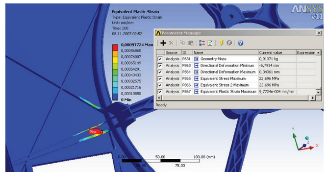
Identification of design details affecting most fatigue lifetime
